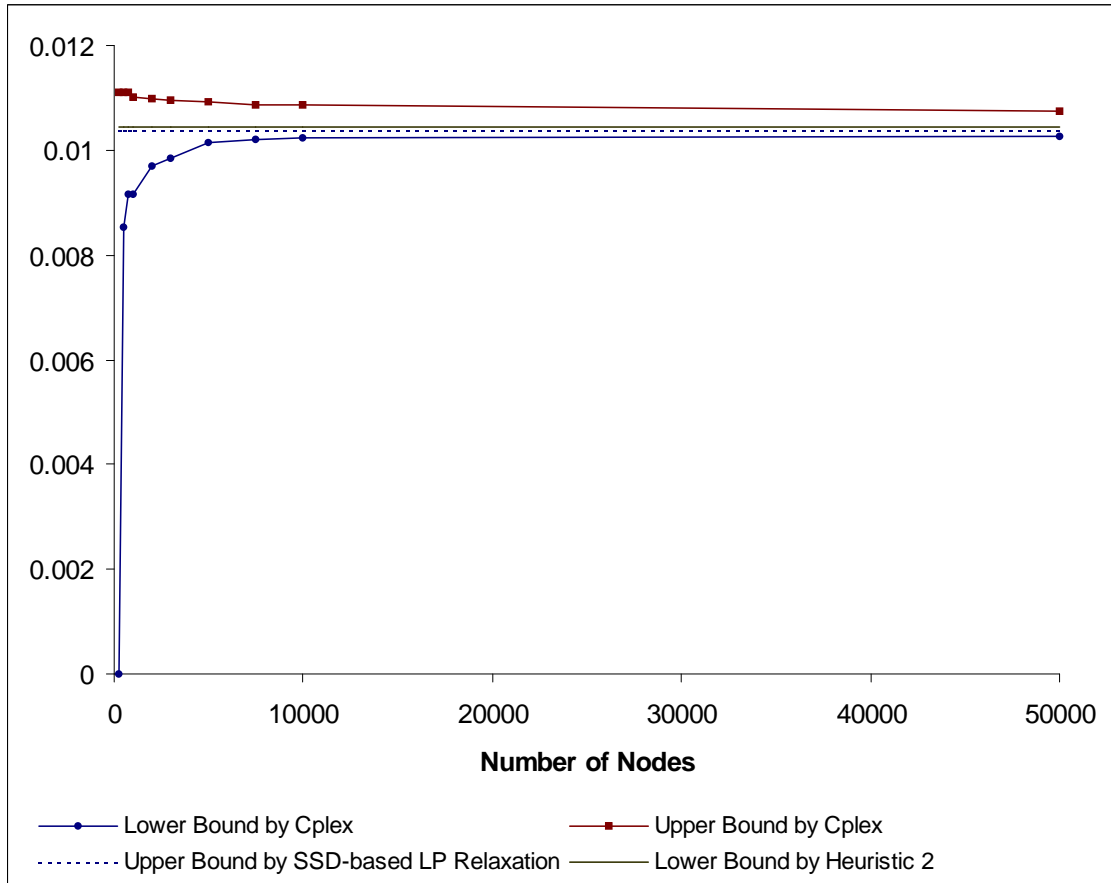
Figure 7: Upper and Lower Bounds on the Optimal Objective Function Value.
