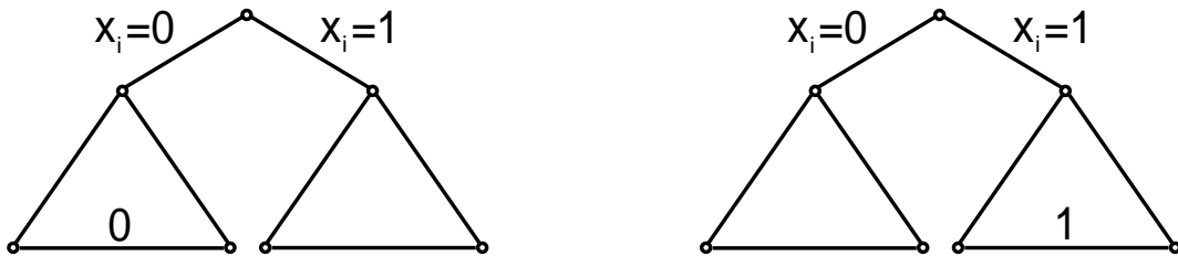
Figure 2: Condition (??) on the left and condition (??) on the right in a branching tree.
