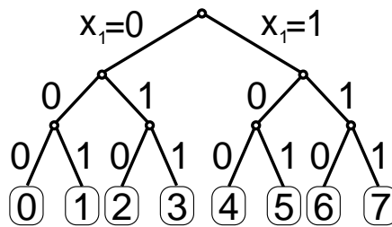
Figure 1: A branching tree on 3 variables.
