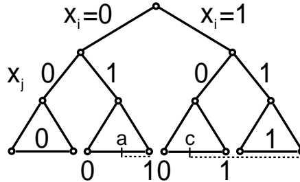
Figure 3: A branching tree of a positive 2-interval function, which is represented by intervals [a, 2^{n-1} - 1], [c, 2^n - 1] and in which no index of a variable satisfies conditions (??) and (??). The pair of variables x_i, x_j satisfies Lemma ??.
