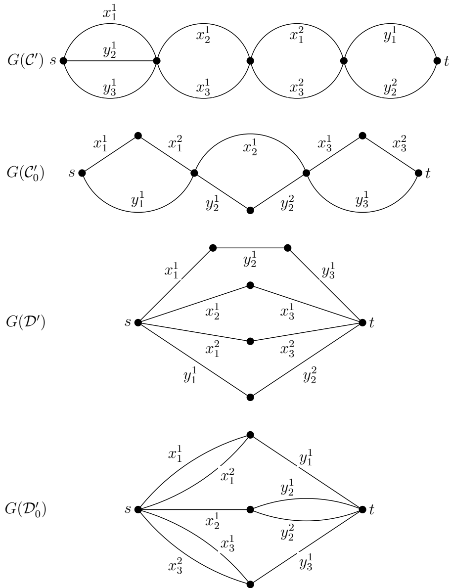
Figure 4: Four labeled graphs corresponding to the CNF \mathcal{C} .
