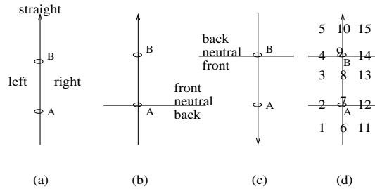
Figure 3: The partition of the universe of 2D positions on which is based Freksa's relative orientation calculus.
