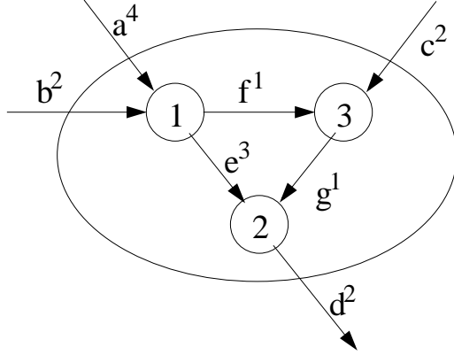
Figure 2: Part of a fractional solution containing a violated HECC.
