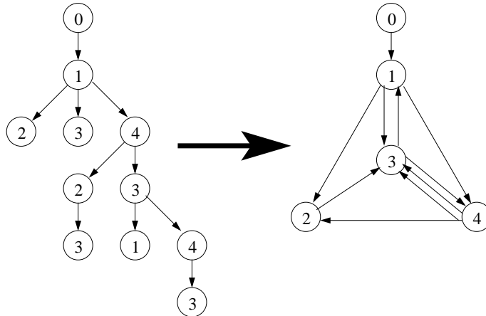
Figure 1: A q -arb and its corresponding multigraph.
