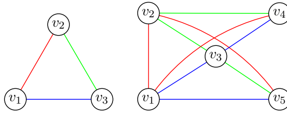
Figure 29: Settling \Delta .
