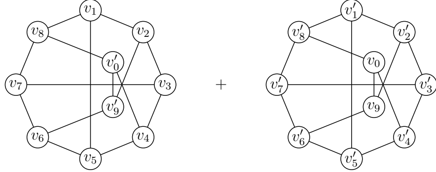
Figure 28: The graph 2\mathcal{P} , isomorphic to 2G_{10} by exchanging v_0, v'_0 and v_9, v'_9 .
