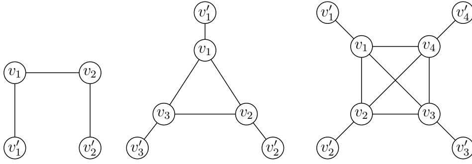
Figure 4: Combs S_k , for k = 2, 3 and 4
