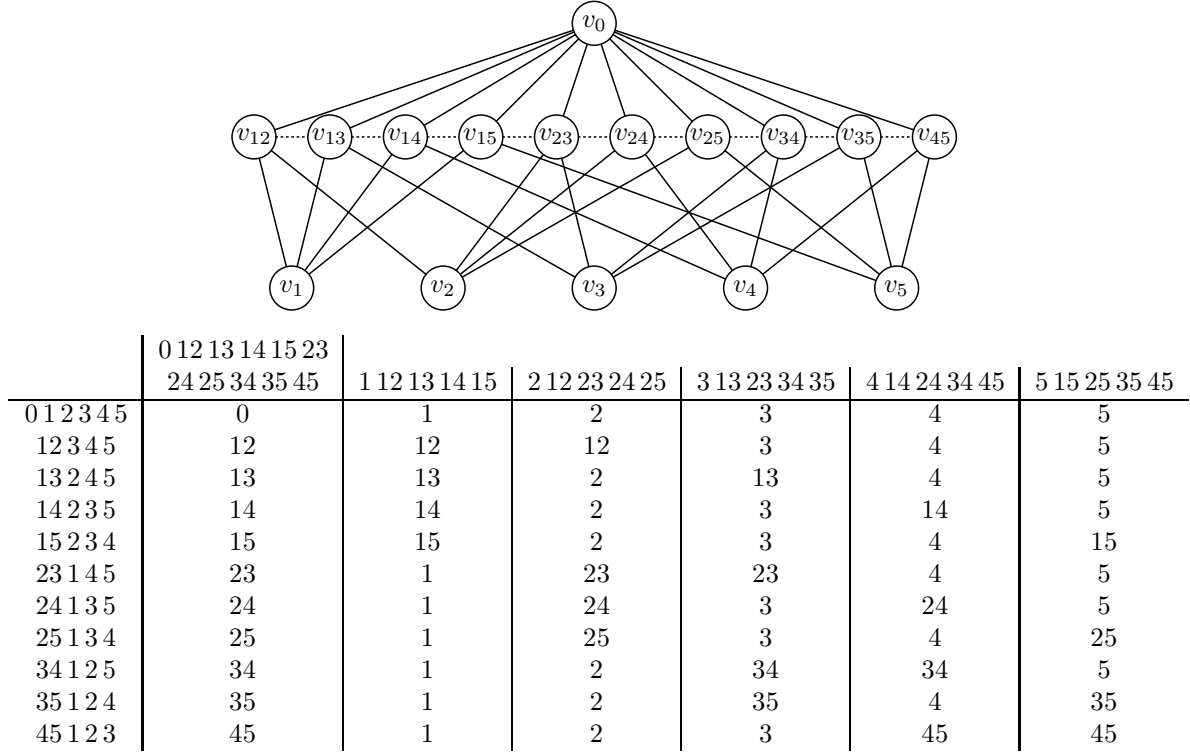
Figure 10: Settled G(5, 1, 2) .
