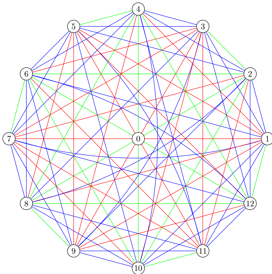
Figure 37: 6-flower example.
