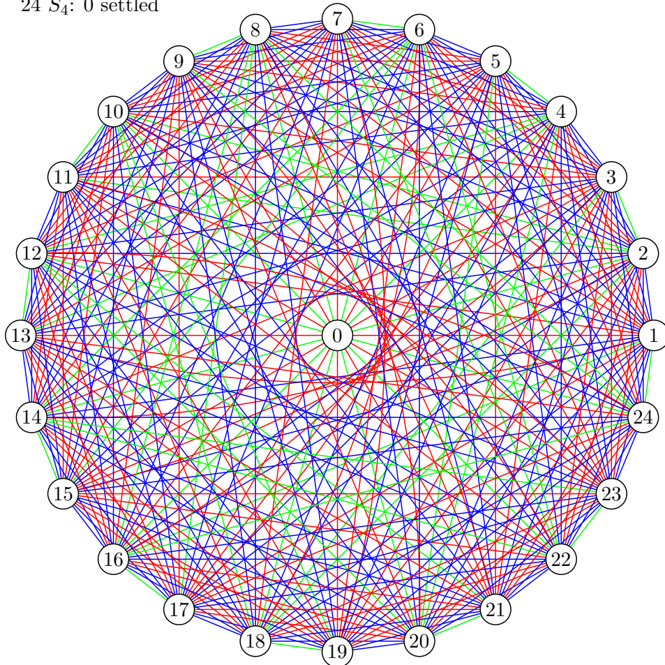
Figure 43: 12-flower example.
