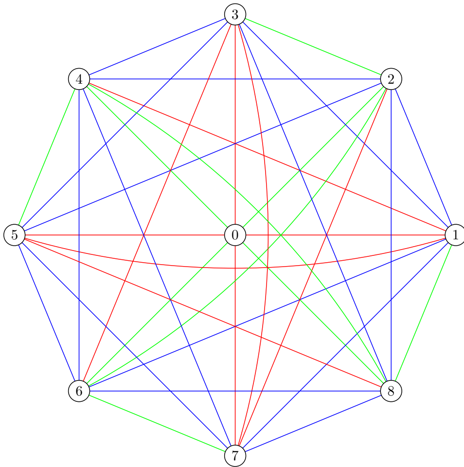
Figure 35: 4-flower example.
