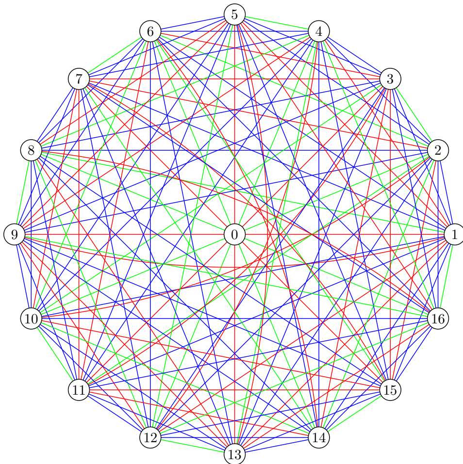
Figure 39: 8-flower example.
