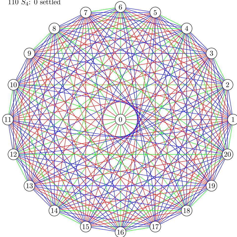
Figure 41: 10-flower example.
