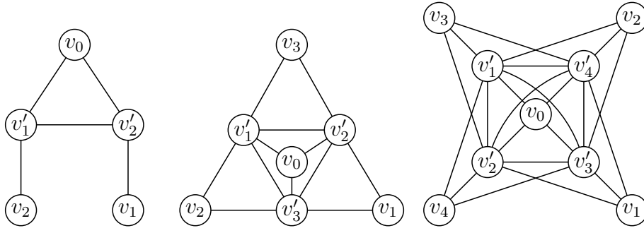
Figure 7: Settled anti-combs \overline{S_k} , for k = 2, 3 and 4 .
